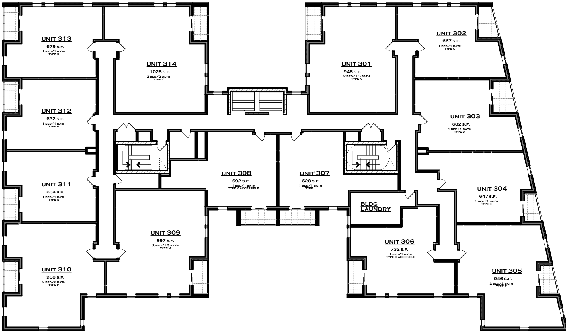
3RD FLOOR PLAN
