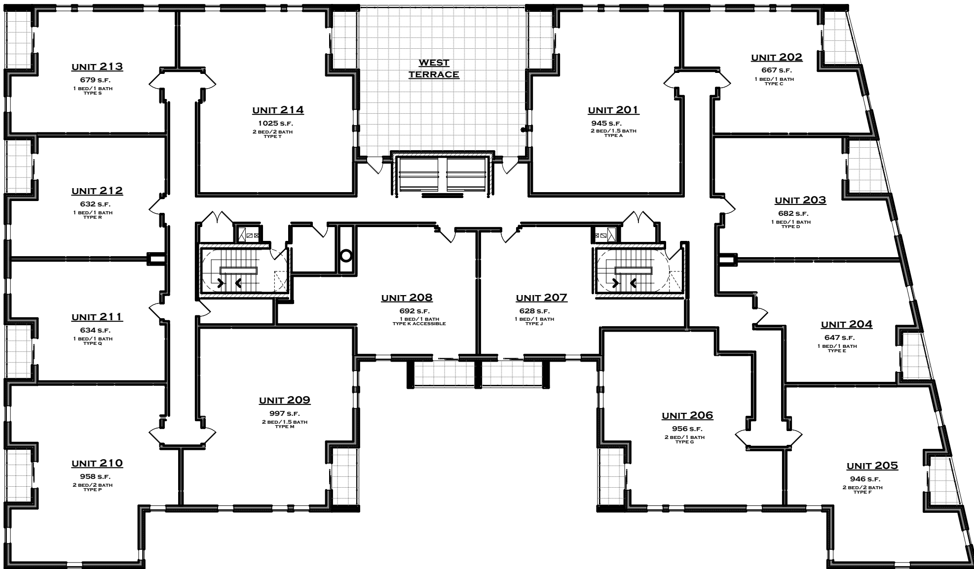
2ND FLOOR PLAN
